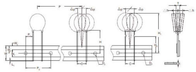
Figure 1 - PTR060V0010-PTR060V0185
